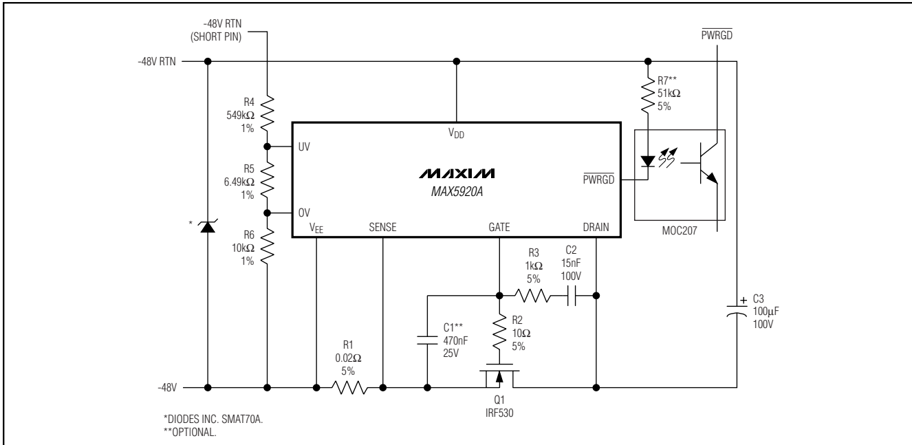
Figure 14. Using PWRGD to Drive an Optoisolator
