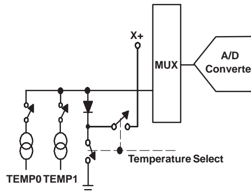
Figure 25. Functional Block Diagram of Temperature Measurement Mode
