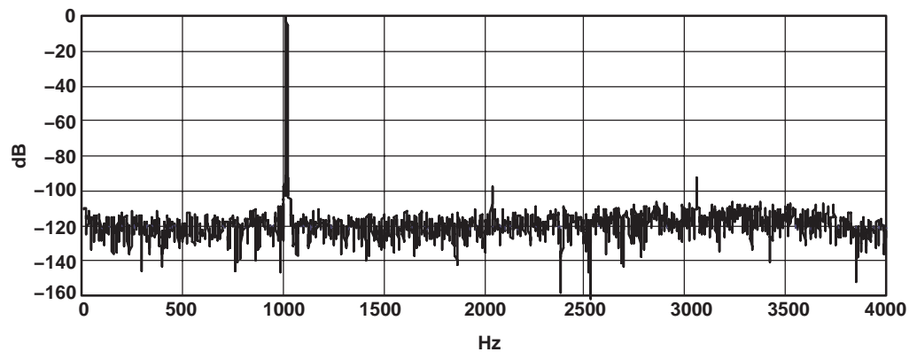
Figure 7. ADC FFT Plot at 8 kps ( T_A = 25^\circ\text{C} , -1 dB, 1 kHz Input, AVDD = 3.3 V)
