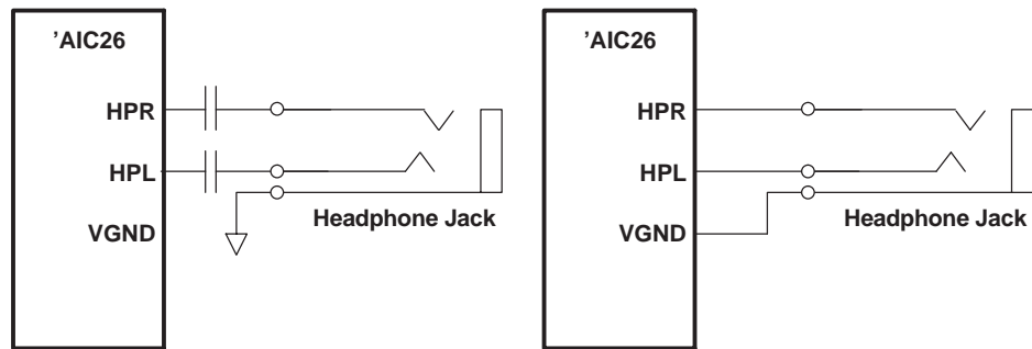
Figure 21. Headphone Configurations, AC-Coupled (left) and Capless (right)
