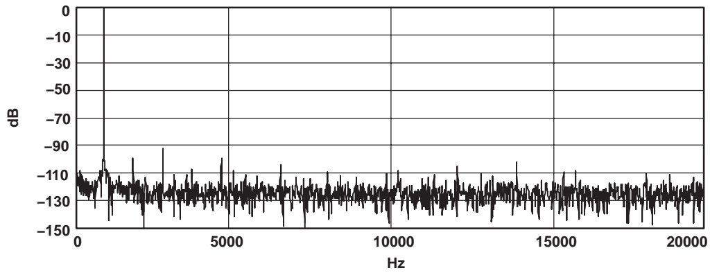
Figure 11. DAC FFT Plot ( T_A = 25^\circ\text{C} , 48 ksp/s, -1 dB, 1 kHz Input, AVDD = DRVDD = 3.3 V, DVDD = 1.8 V, R_L = 16 \Omega )
