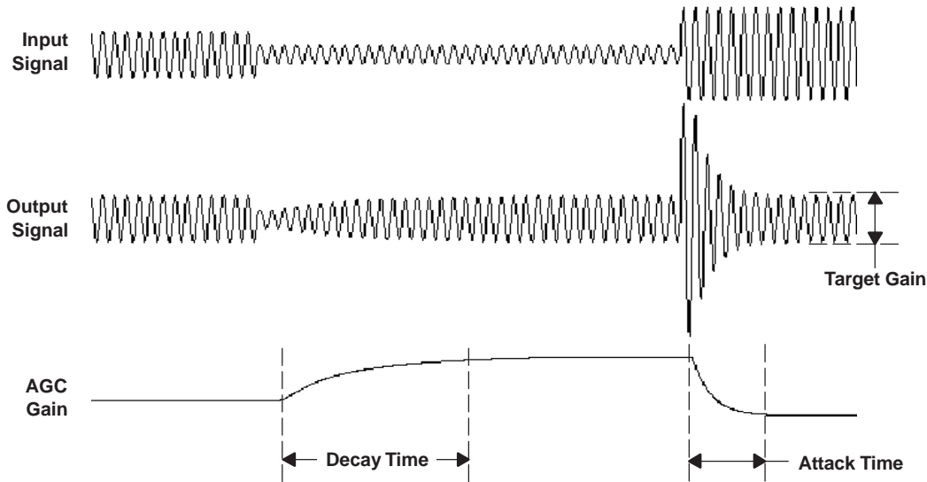
Figure 18. AGC Characteristics
