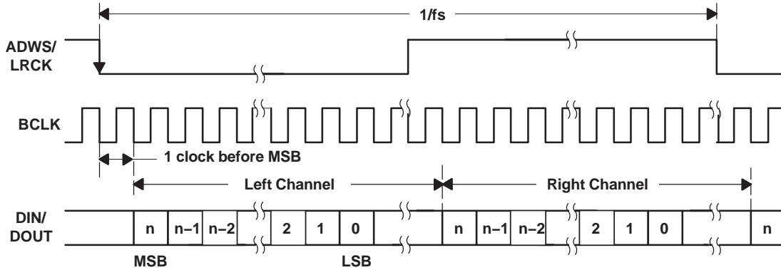
Figure 16. Timing Diagram for I 2 S Mode
