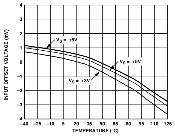
Figure 41. Input Offset Voltage vs. Temperature
