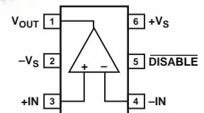
Figure 2. SC70-6 (KS)
