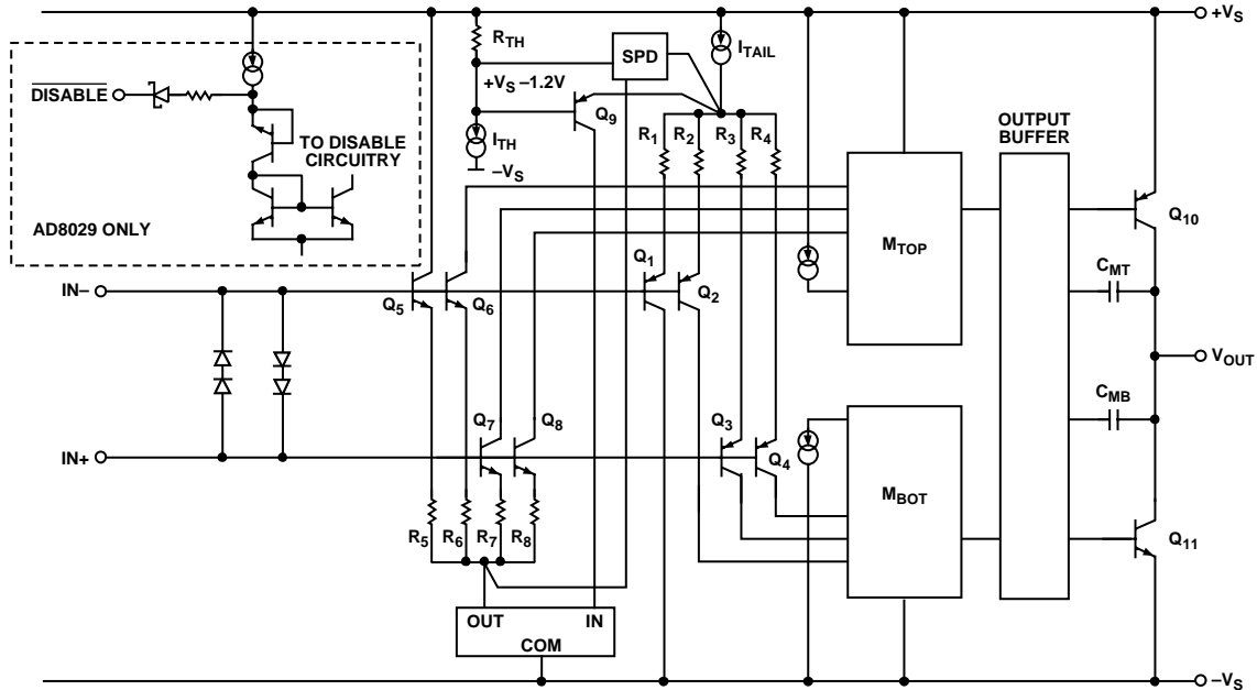
Figure 50. Simplified Schematic
