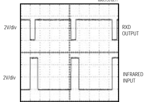
RXD OUTPUT vs. INFRARED INPUT
