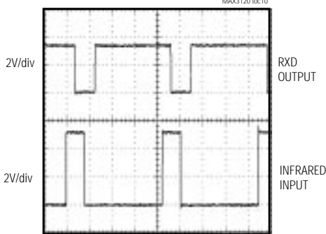
RXD OUTPUT vs. INFRARED INPUT
