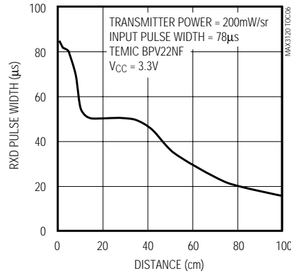
RXD OUTPUT PULSE WIDTH vs. DISTANCE
