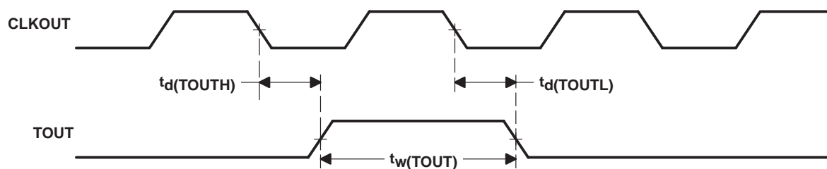
Figure 20. TOUT Timing
