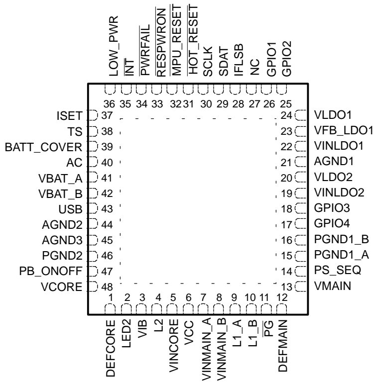
RGZ PACKAGE (TOP VIEW)
