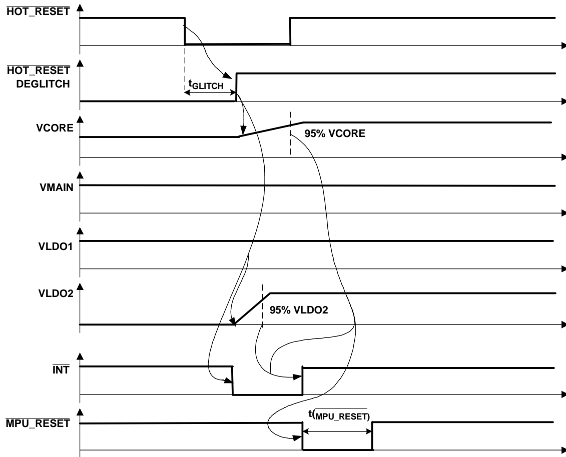
Figure 37. State 3 to State 2 Transition ( HOT_RESET Activated, See Interrupt Management Section for INT Behavior)
