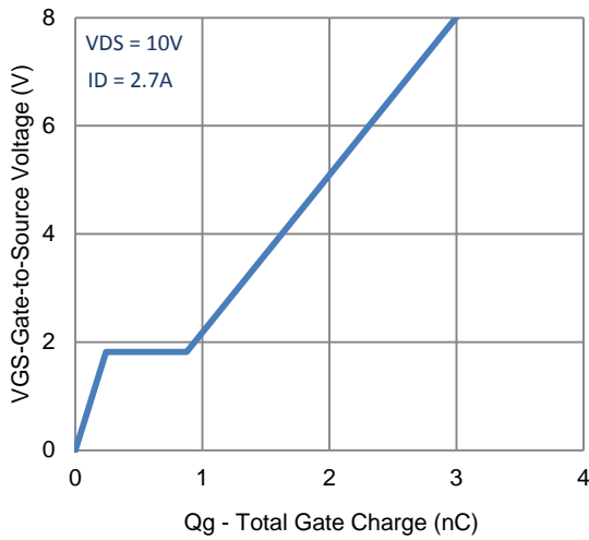
7. Gate Charge
