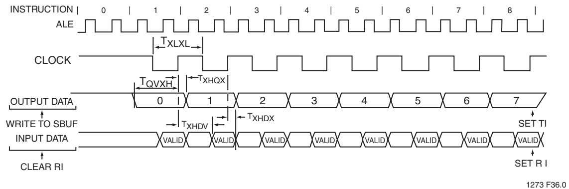
FIGURE 14-7: Shift Register Mode Timing Waveforms
