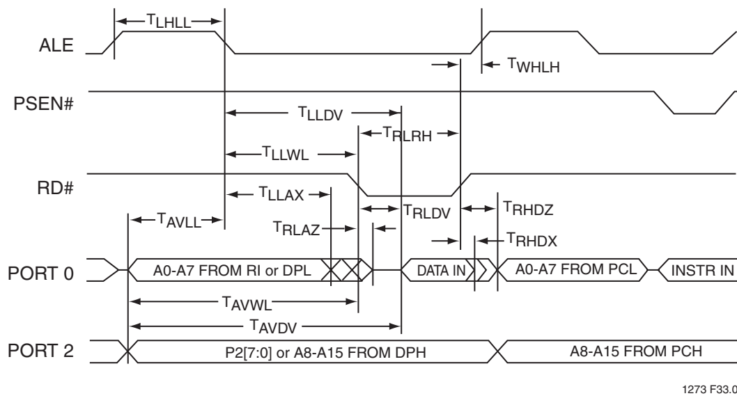
FIGURE 14-4: External Data Memory Read Cycle
