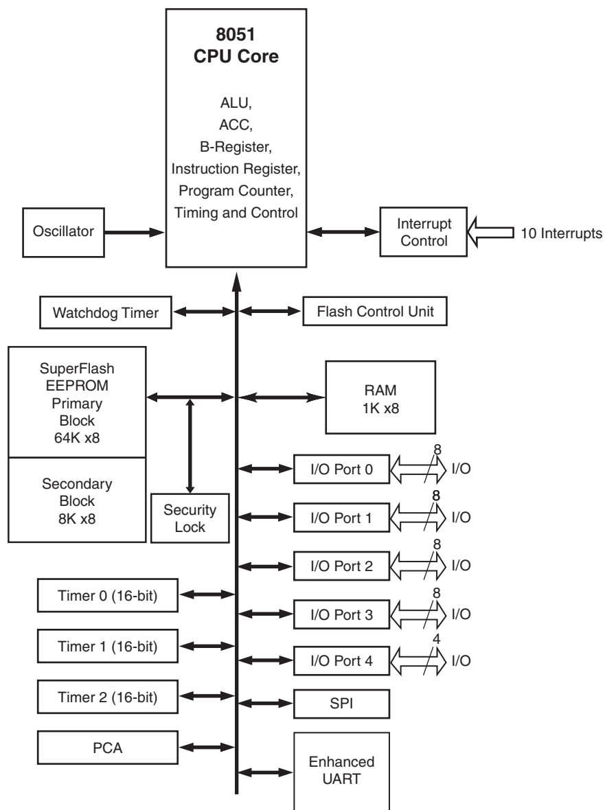
FIGURE 1-1: Functional Block Diagram
