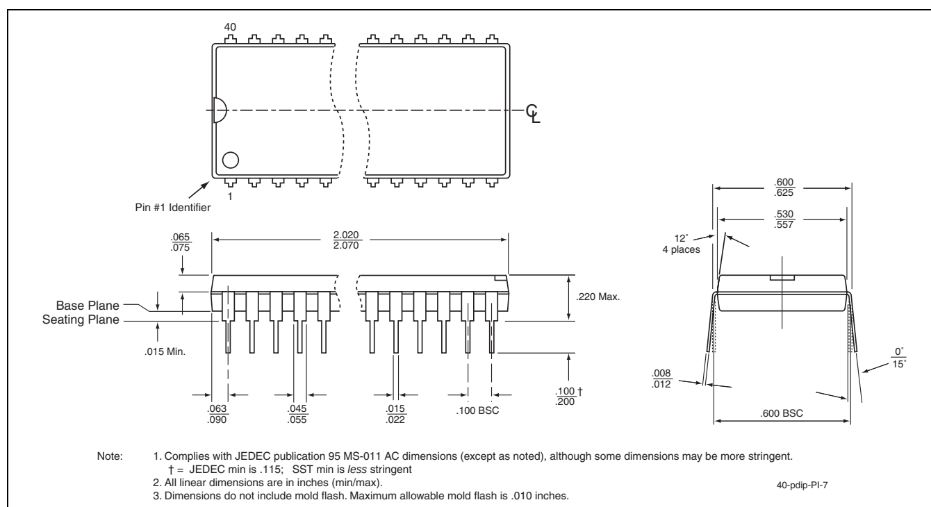
FIGURE 16-2: 40-pin Plastic Dual In-line Pins (PDIP) SST Package Code: PI
