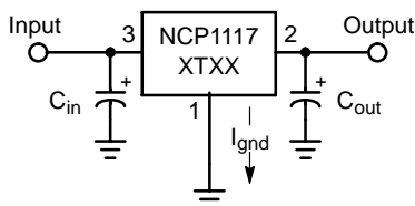
Figure 20. Fixed Output Regulator
