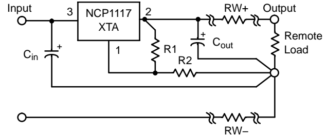
Figure 23. Load Sensing
