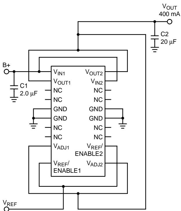
Figure 13. 400 mA Loading
