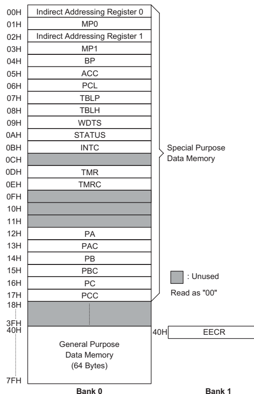
RAM Mapping
