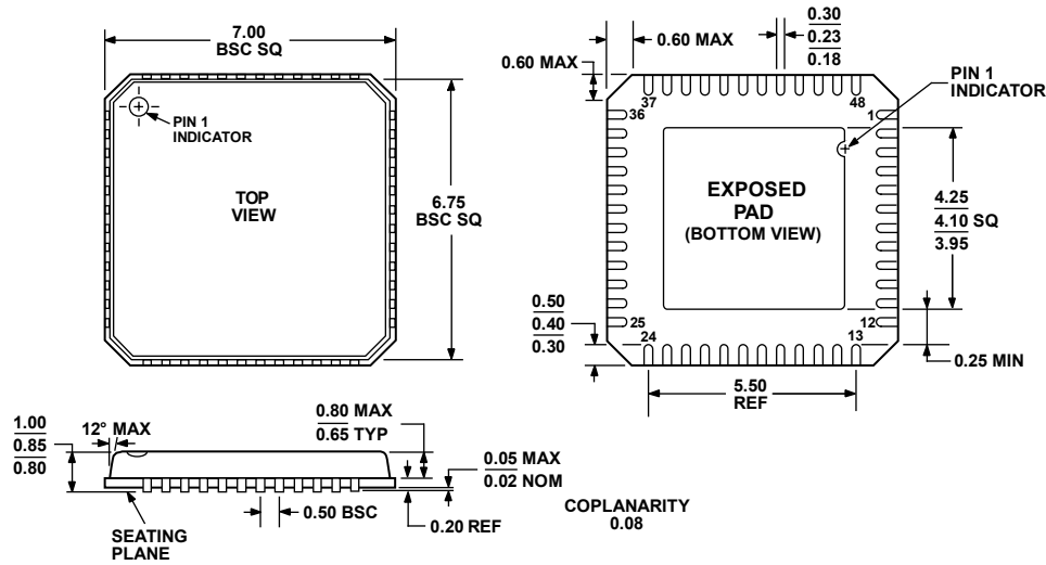
Figure 71. 48-Lead Frame Chip Scale Package [LFCSP_VQ] 7 mm × 7 mm Body, Very Thin Quad (CP-48-3) Dimensions shown in millimeters
