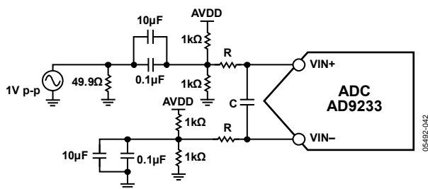
Figure 41. Single-Ended Input Configuration
