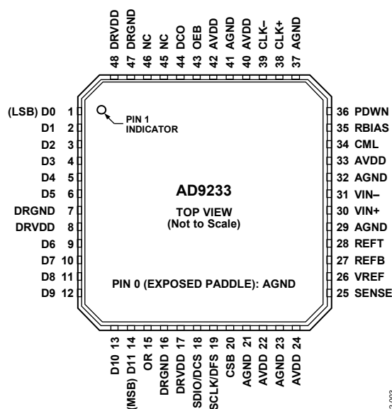
Figure 3. Pin Configuration
