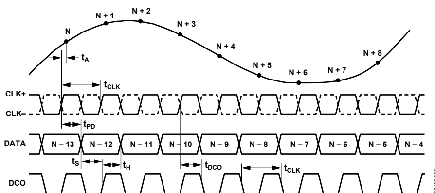
Figure 2. Timing Diagram
