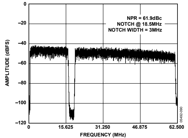
Figure 29. AD9233-125 Noise Power Ratio
