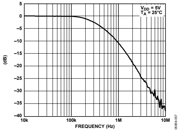
Figure 49. Multiplying Bandwidth
