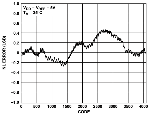
Figure 6. INL AD5627, External Reference
