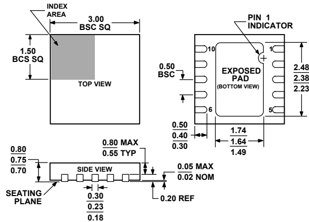
Figure 67. 10-Lead Lead Frame Chip Scale Package [LFCSP_WD] 3 mm x 3 mm Body, Very Very Thin, Dual Lead (CP-10-9) Dimensions shown in millimeters
