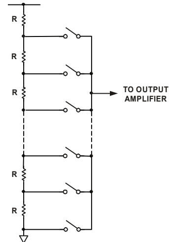
Figure 51. Resistor String
