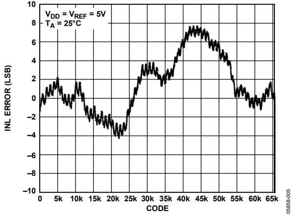
Figure 4. INL AD5667, External Reference
