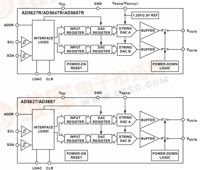
Figure 1. Functional Block Diagrams
