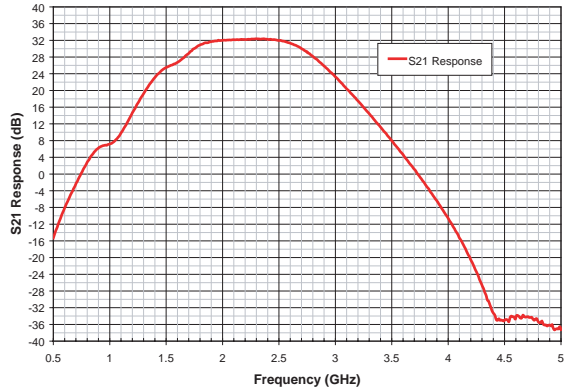
Figure 30: 2.4 GHz S21 Response Across Frequency ( V_{CC} = +3.3\text{ V} , T_C = 25^\circ\text{C} )
