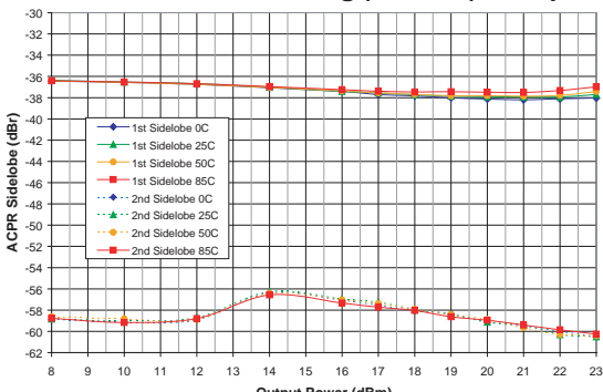
Figure 15: ACPR vs. Output Power Across Temp (Freq = 2.45 GHz, V CC = +3.3 V) 802.11b Gaussian Filtering (BT = 0.5), 1 Mbps
