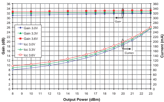
Figure 13: Gain and I CC vs. Output Power Across Power Supply Voltage (Freq = 2.45 GHz, T C = 25°C) 802.11b Gaussian Filtering (BT = 0.5), 1 Mbps
