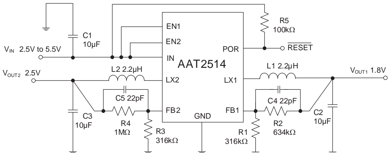
Figure 1: AAT2514 Typical Application Circuit.
