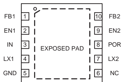
AAT2514-IDE TDFN33-10 (Top View)
