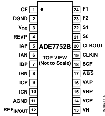
Figure 3. Pin Configuration
