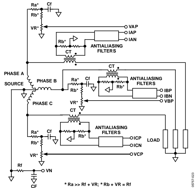
Figure 22. 3-Phase 4-Wire Meter Connection with ADE7752B
