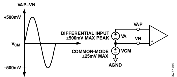
Figure 19. Maximum Signal Levels, Voltage Channel
