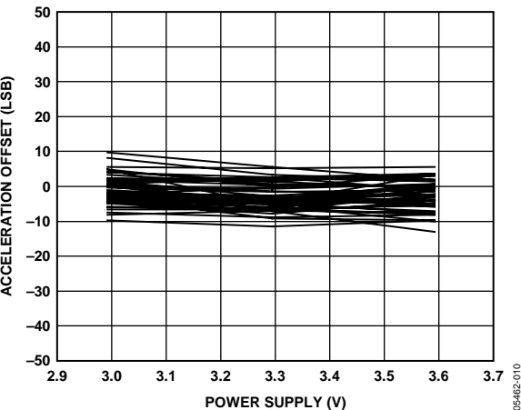
Figure 10. Acceleration Offset vs. Supply at 25°C
