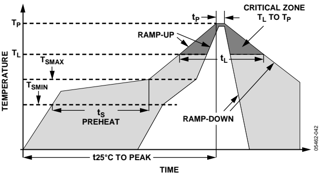
Figure 41. Acceptable Solder Reflow Profiles
