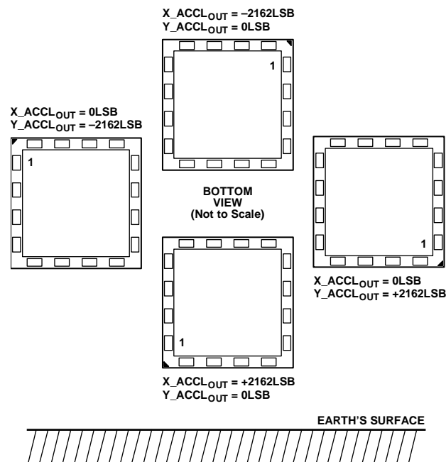
Figure 39. Output Response vs. Orientation
