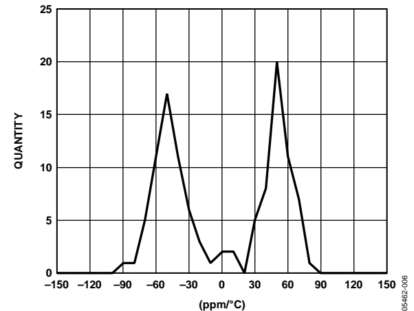
Figure 6. Acceleration Sensitivity Tempco Histogram at 3.3 V
