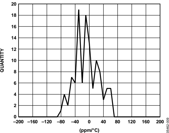
Figure 9. Acceleration Offset Tempco Histogram at 3.3 V
