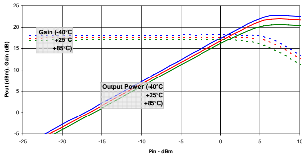
Figure 4. Output Power and Gain vs. Temperature
