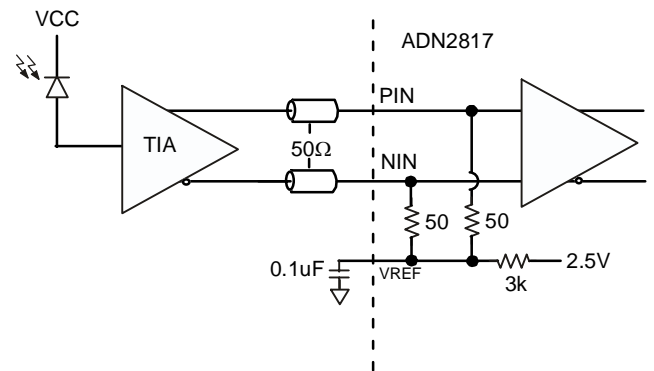
Figure 28. DC-Coupled Application
