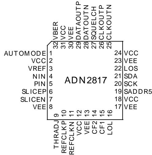
Figure 4. Pin Configuration
