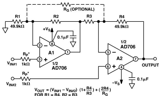
Figure 24. A Two Op-Amp Instrumentation Amplifier
