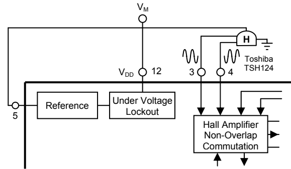
Figure 21- Reference Powered Unbuffered Hall
