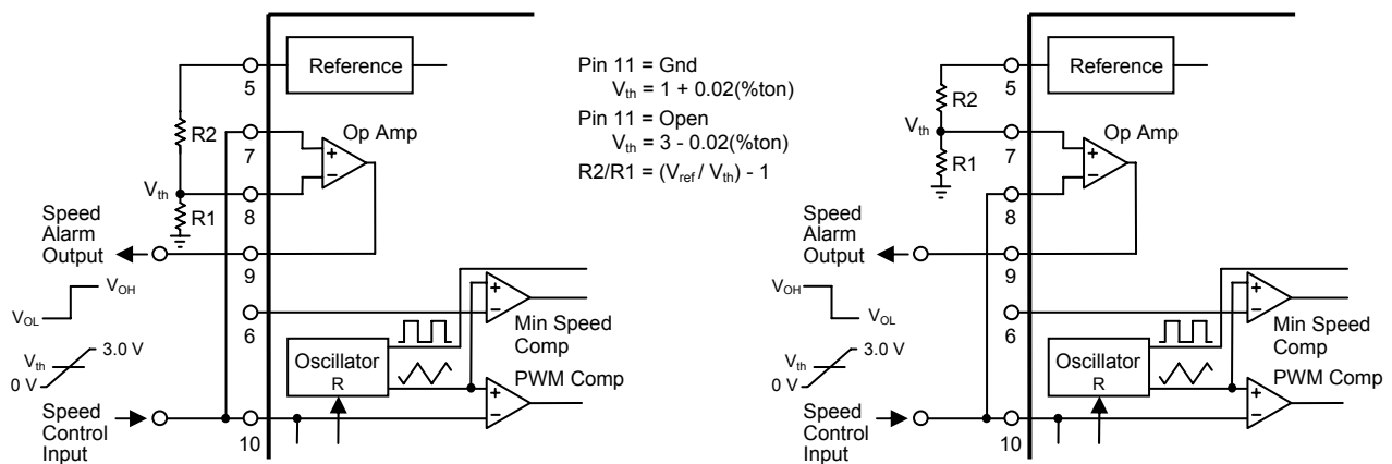
Figure 42- Speed Control Alarm
