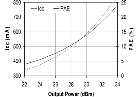
PAE / I_{cc} vs. Output Power
