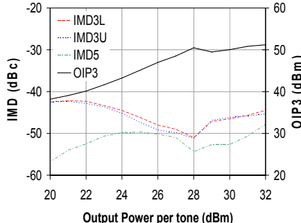
IMD3, IMD5, OIP3 vs. Output Power
