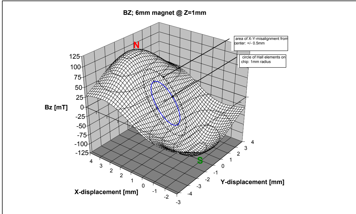
Figure 31. Vertical Magnetic Field Distribution of a Cylindrical 6mm \varnothing Diametric Magnetized Magnet at 1mm Gap
