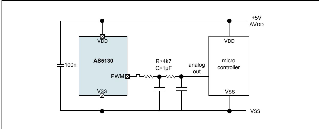
Figure 9. Ratiometric Analog Output
