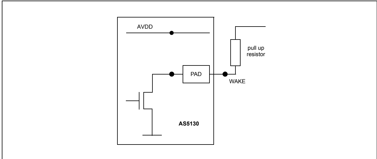
Figure 20. WAKE Output Pin
