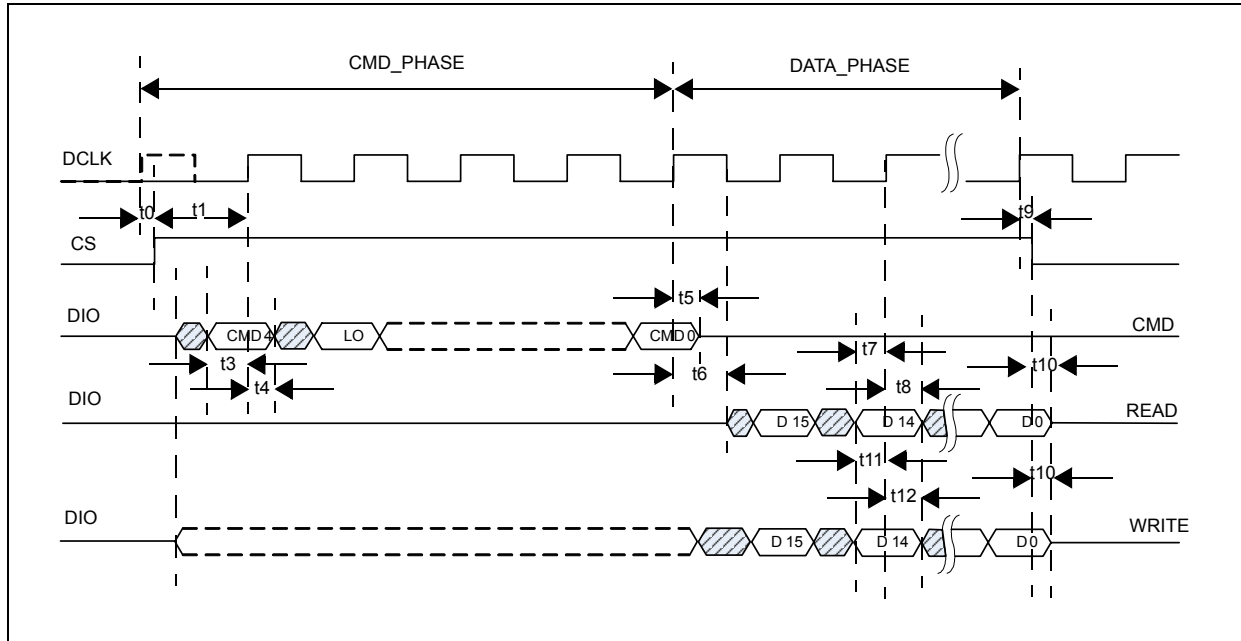
Figure 4. Normal Operation Mode
