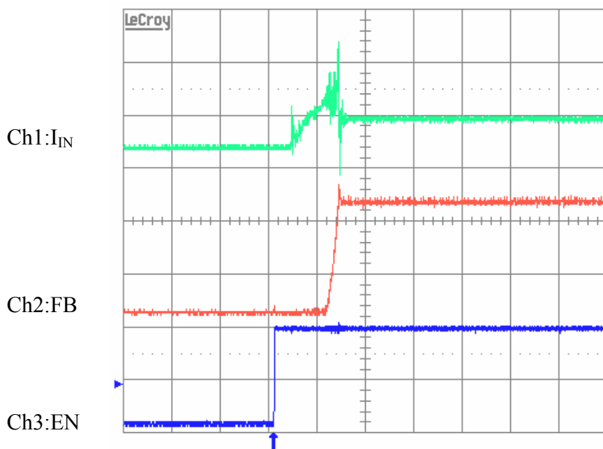
Ch1:I IN : 200mA/div , Ch2:FB: 100mV/div , Ch3:ENABLE:2V/div ,0.5mS/div
