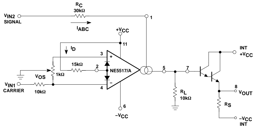
Figure 25. Amplitude Modulator
