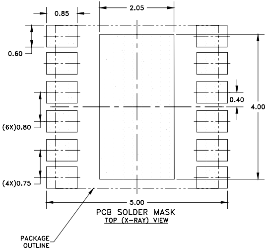
Figure 17: Land Pattern
