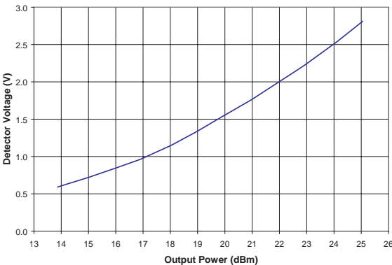
Figure 7: Detector Voltage vs. Output Power ( T_C = +25\text{ }^\circ\text{C} , V_{CC} = +6.0\text{ V} , V_{BIAS} = +3.0\text{ V} , f = 3.5\text{ GHz} , 54 Mbps OFDM Modulation)
