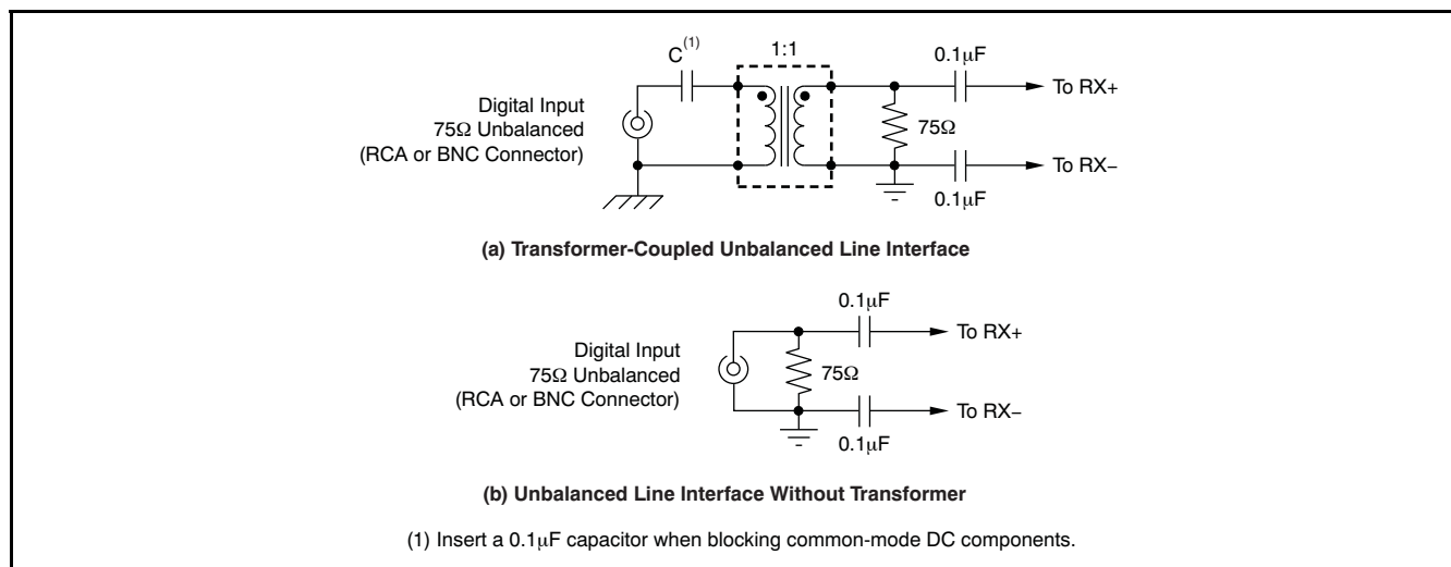
Figure 26. Unbalanced Line Input Interfaces
