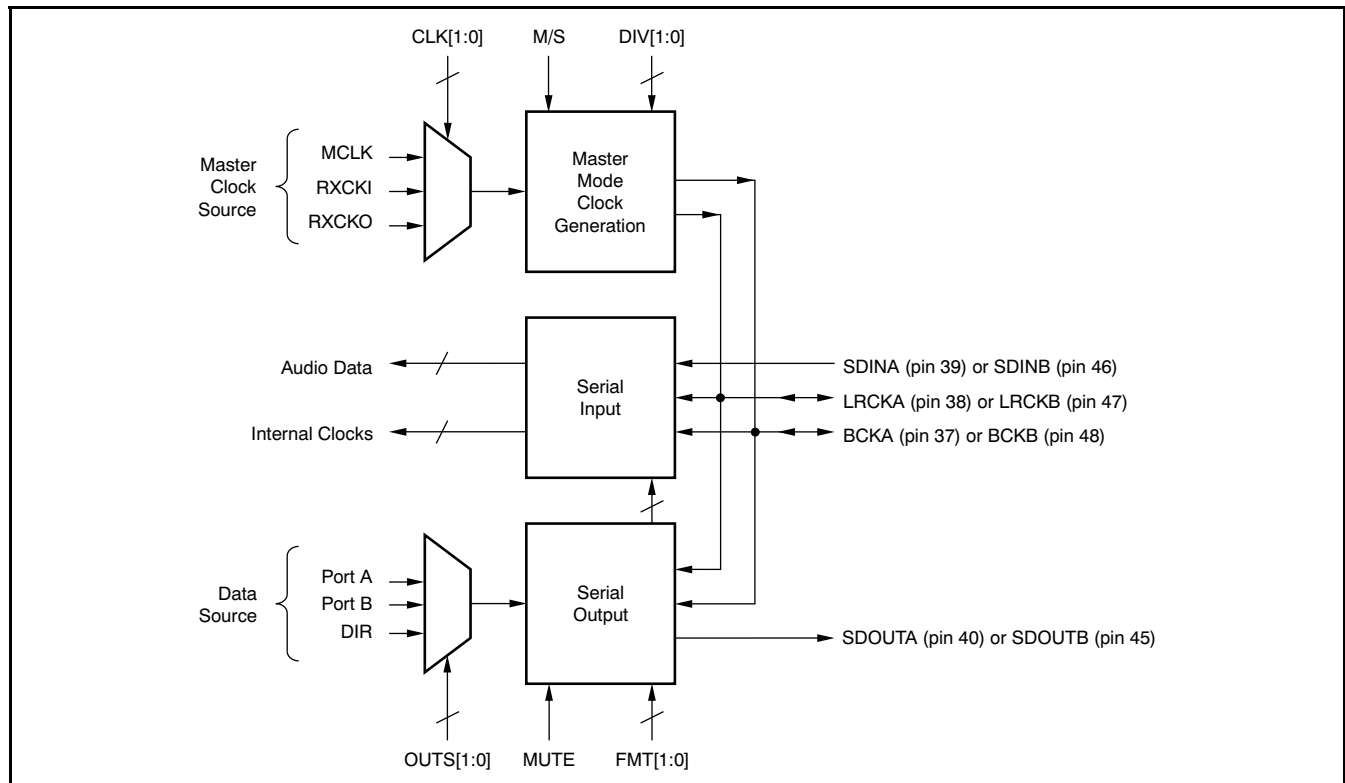
Figure 6. Audio Serial Port Block Diagram
