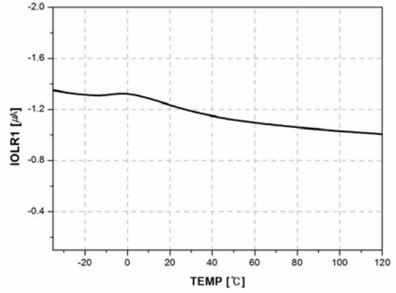
Figure 28. Error Amp. Source Current 1 vs. Temp.
