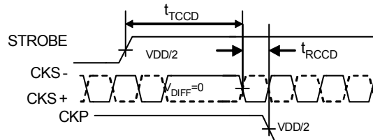
Figure 9. Clock Propagation Delay
