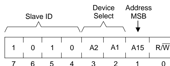
Figure 4. Slave Address
