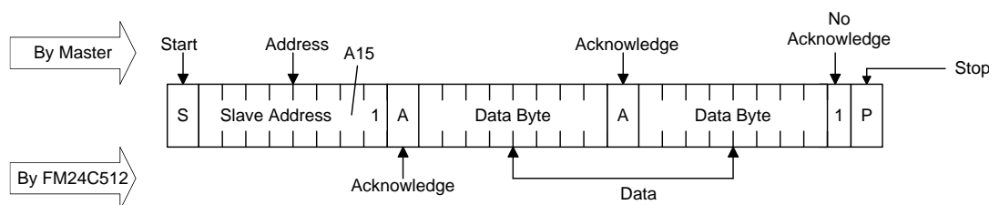
Figure 8. Sequential Read
