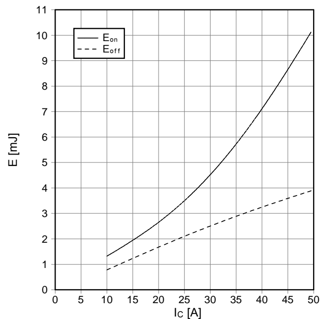
Schaltverluste IGBT-Wechselr. (typisch) switching losses IGBT-inverter (typical) E_{on} = f(I_c) , E_{off} = f(I_c) V_{GE} = \pm 15\text{ V} , R_{Gon} = 36\ \Omega , R_{Goff} = 36\ \Omega , V_{CE} = 600\text{ V} , T_{vj} = 125^\circ\text{C}
