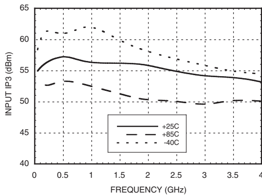
Input IP3 vs. Temperature, Vctl = 0/+3V
