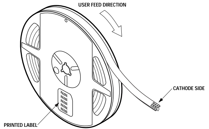
Figure 10. Reeling orientation.
