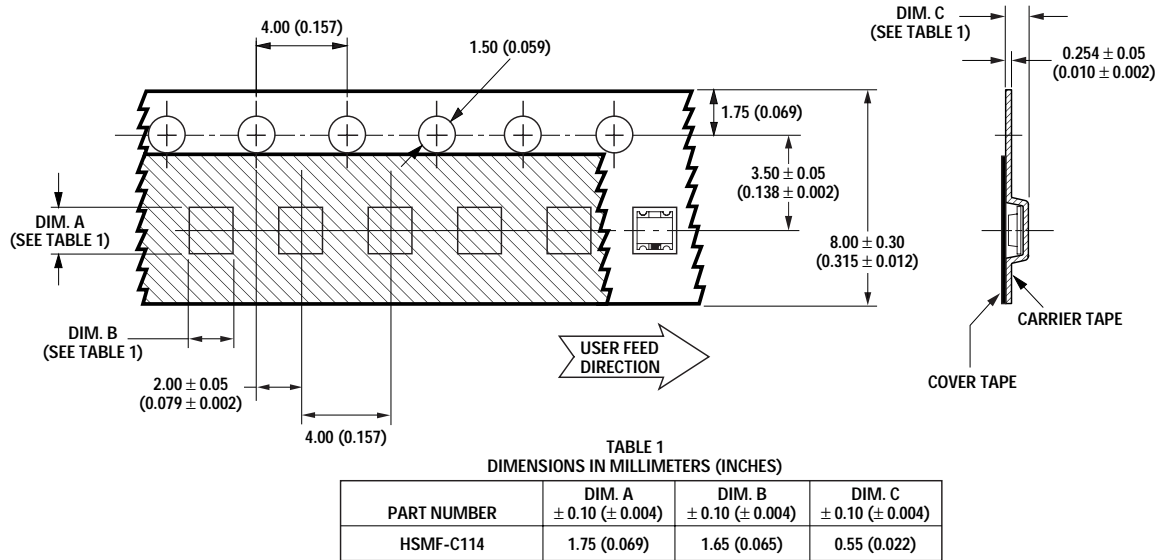
Figure 12. Tape dimensions.
