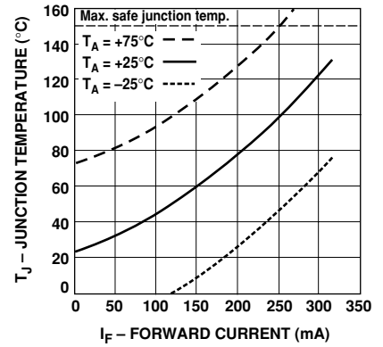
Figure 3. Junction Temperature vs. Forward Current as a Function of Heat Sink Temperature for the HSMS-2700 and HSMS-2702.
