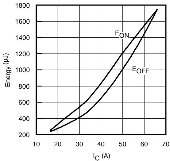
Fig. 11 - Typ. Energy Loss vs. I_C
