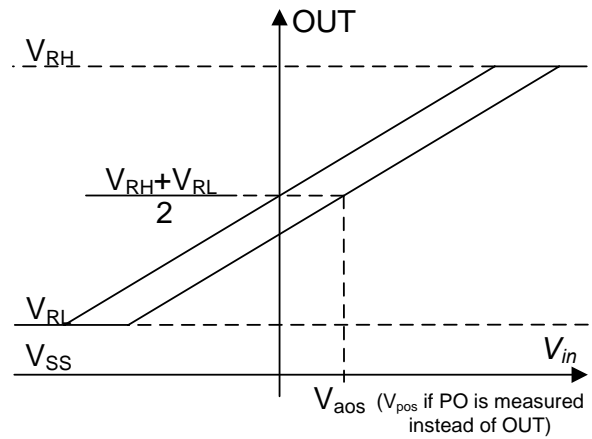
Figure 10: Input offset definition
