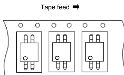
Figure1 Device Orientation
