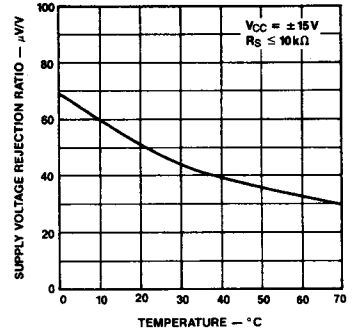
Supply Voltage Rejection Ratio vs Temperature (μA715C)
