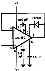
Voltage Follower (Note 1)
