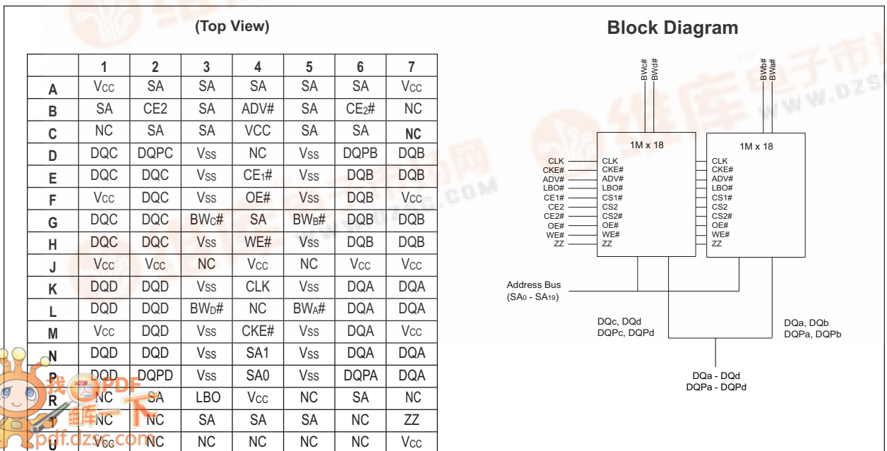
FIGURE 1 – PIN CONFIGURATION
