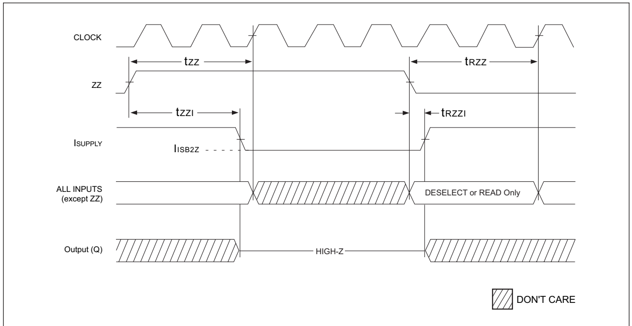
FIGURE 2 – SNOOZE MODE TIMING DIAGRAM
