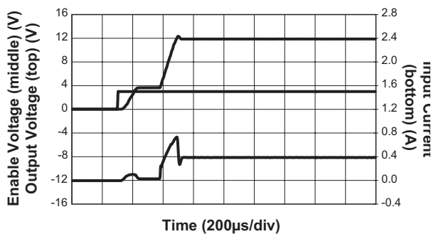
Soft Start (V_{IN} = 3.6V; C_{IN} = 2.2µF; I_{OUT} = 100mA; V_{OUT} = 12V)
