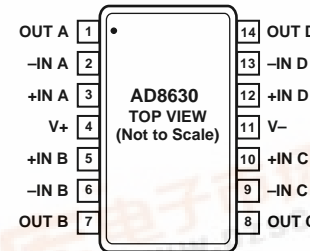
Figure 5. 14-Lead SOIC_N (R-14)
