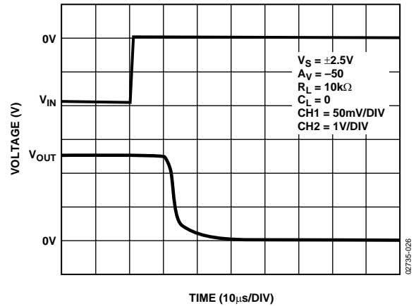
Figure 30. Negative Overtolerance Recovery
