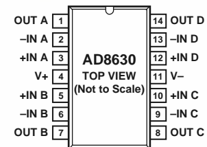
Figure 6. 14-Lead TSSOP (RU-14)
