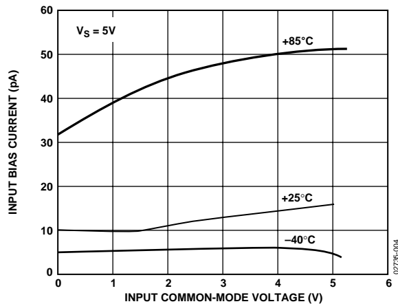
Figure 8. AD8628 Input Bias Current vs. Input Common-Mode
