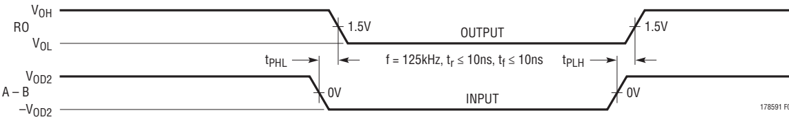
Figure 7. Receiver Propagation Delays
