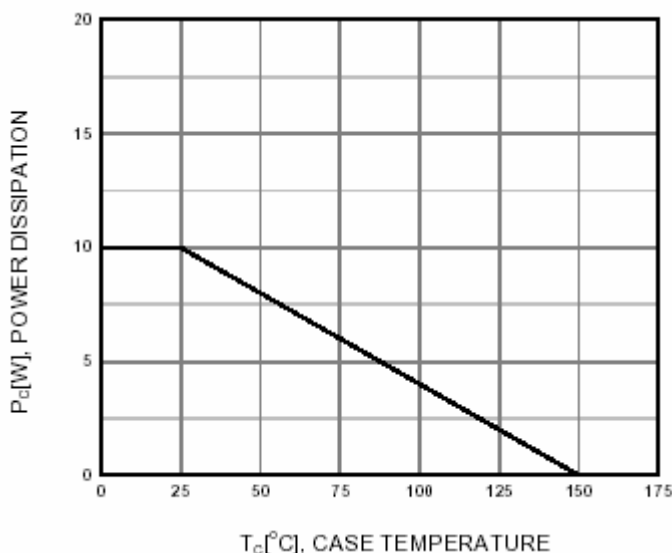
Fig.7 Power Derating
