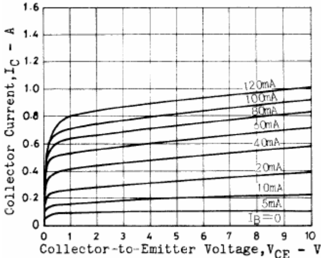
Fig.3 Static Characteristic
