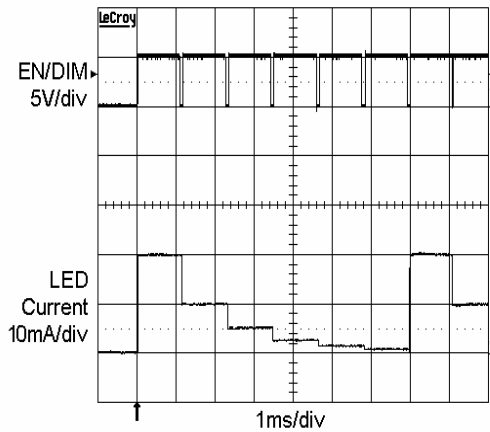
Dimming Waveform
