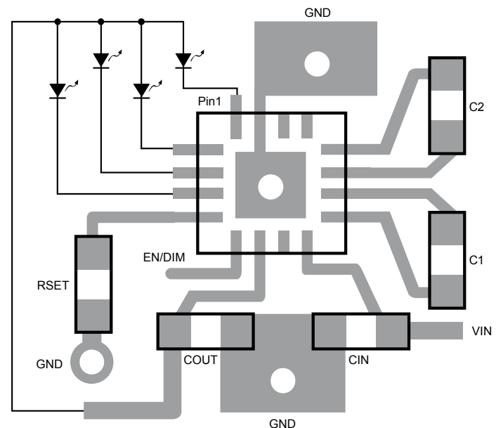
Figure 5. Recommended Layout
