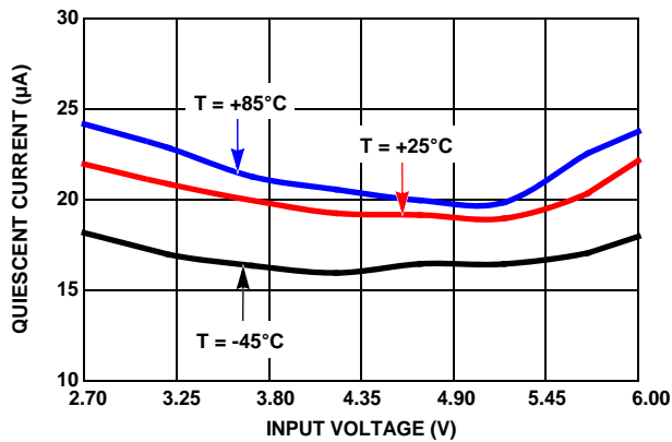
FIGURE 3. INPUT QUIESCIENT CURRENT vs V_{IN} ( V_{OUT} = 2.5\text{V} )
