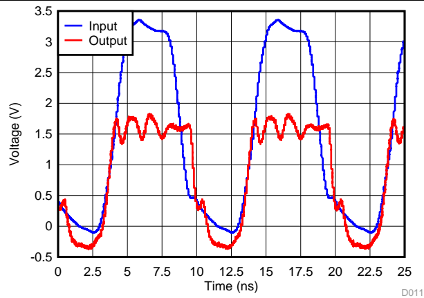
Figure 14. Waveform From TP1 (Pull-up Resistor: 160- \Omega and 50-pF Capacitance 3.3 V to 1.8 V at 100 MHz)
