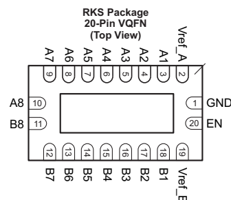
LSF0108
