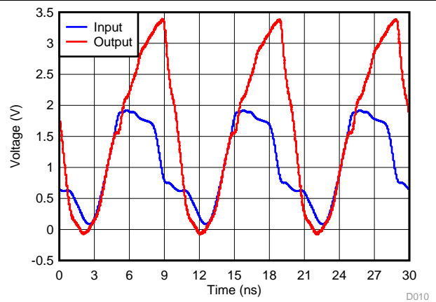
Figure 15. Waveform From TP2 (Pull-up Resistor: 160- \Omega and 50-pF Capacitance 1.8 V to 3.3 V at 100 MHz)
