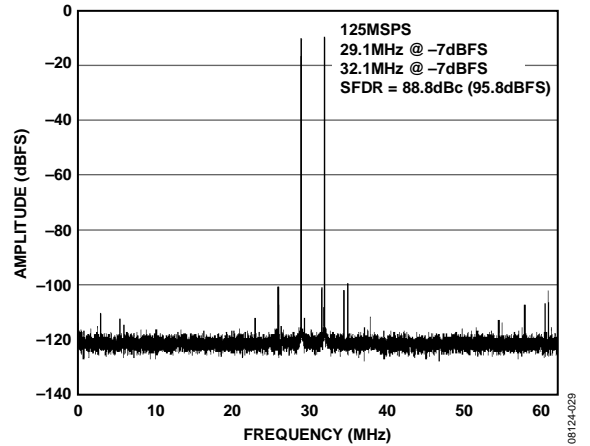
Figure 48. AD9258-125 Two-Tone FFT with f_{IN1} = 29.1 MHz and f_{IN2} = 32.1 MHz
