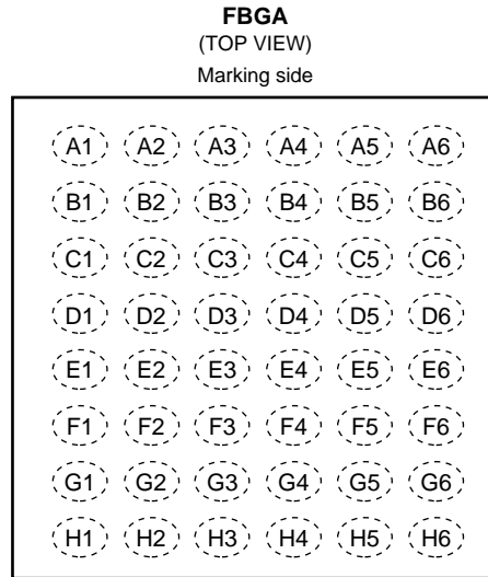
(BGA-48P-M11)
