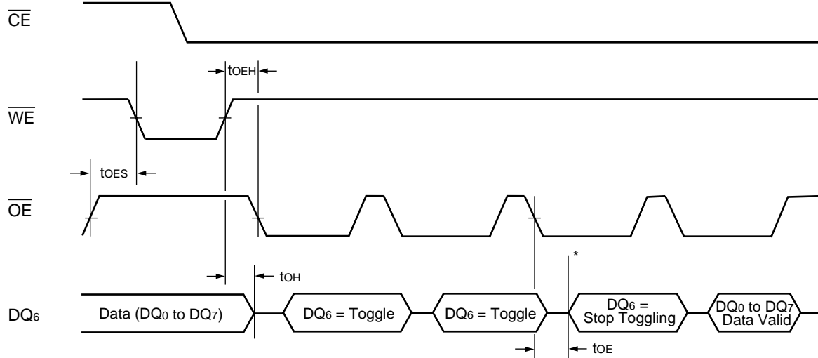
Figure 10 Toggle Bit I during Embedded Algorithm Operation Timing Diagram
