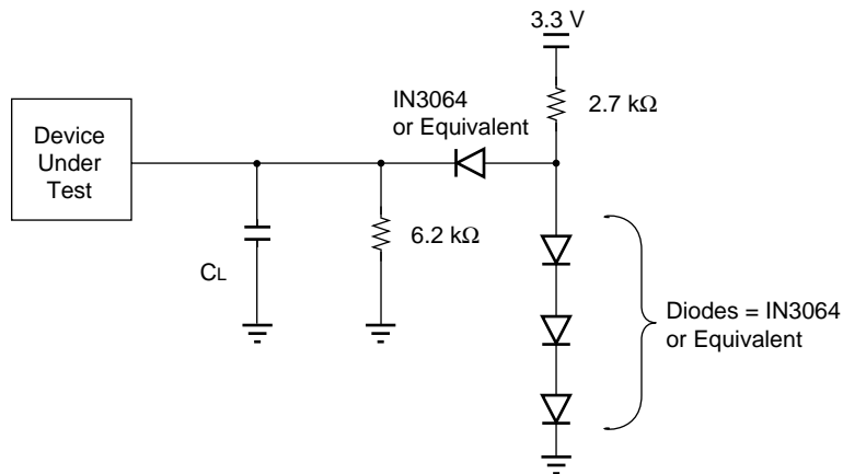
Figure 4 Test Conditions
